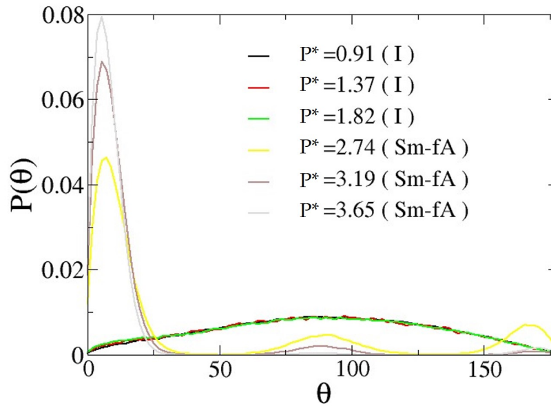
FIGURE 4.13: Distribution of angles between two cylinders of the same G-DNA duplex at different pressures for isotropic ( \beta P v_0 = 0.91, 1.37 , and 1.82 ) and smectic phase ( \beta P v_0 = 3.19 and 3.65 ).
